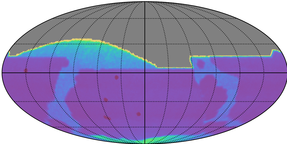
weather_cloudso36v3.4_10yrs : Proper Motion Uncert @ 20.5
