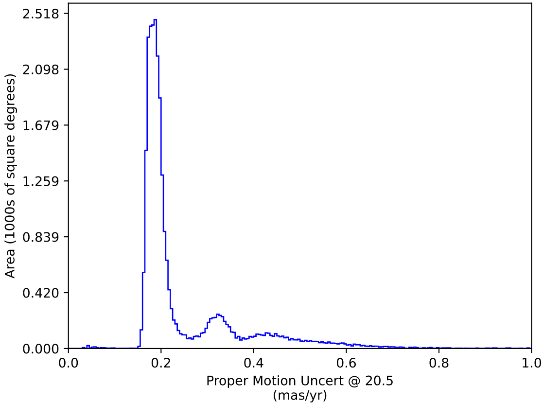
weather_cloudso36v3.4_10yrs : Proper Motion Uncert @ 20.5
