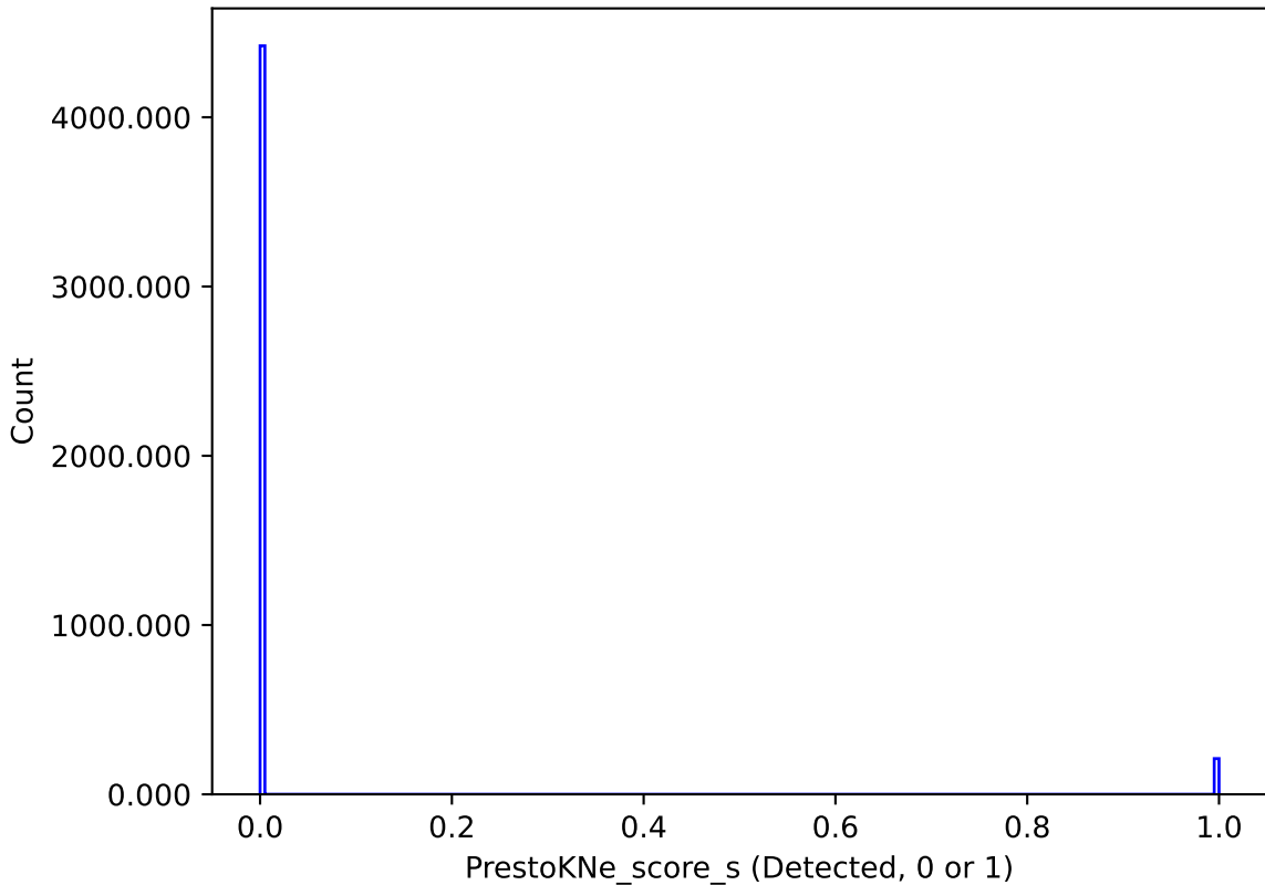
weather_cloudso36v3.4_10yrs : PrestoKNe_score_s
