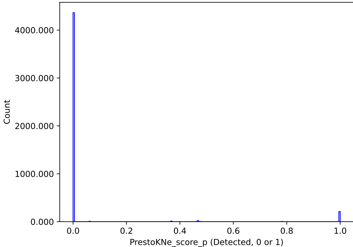
weather_cloudso36v3.4_10yrs : PrestoKNe_score_p
