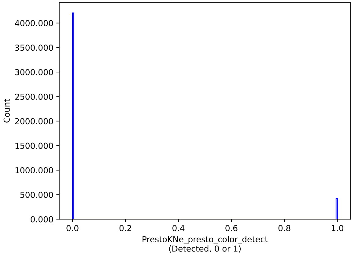
weather_cloudso36v3.4_10yrs : PrestoKNe_presto_color_detect
