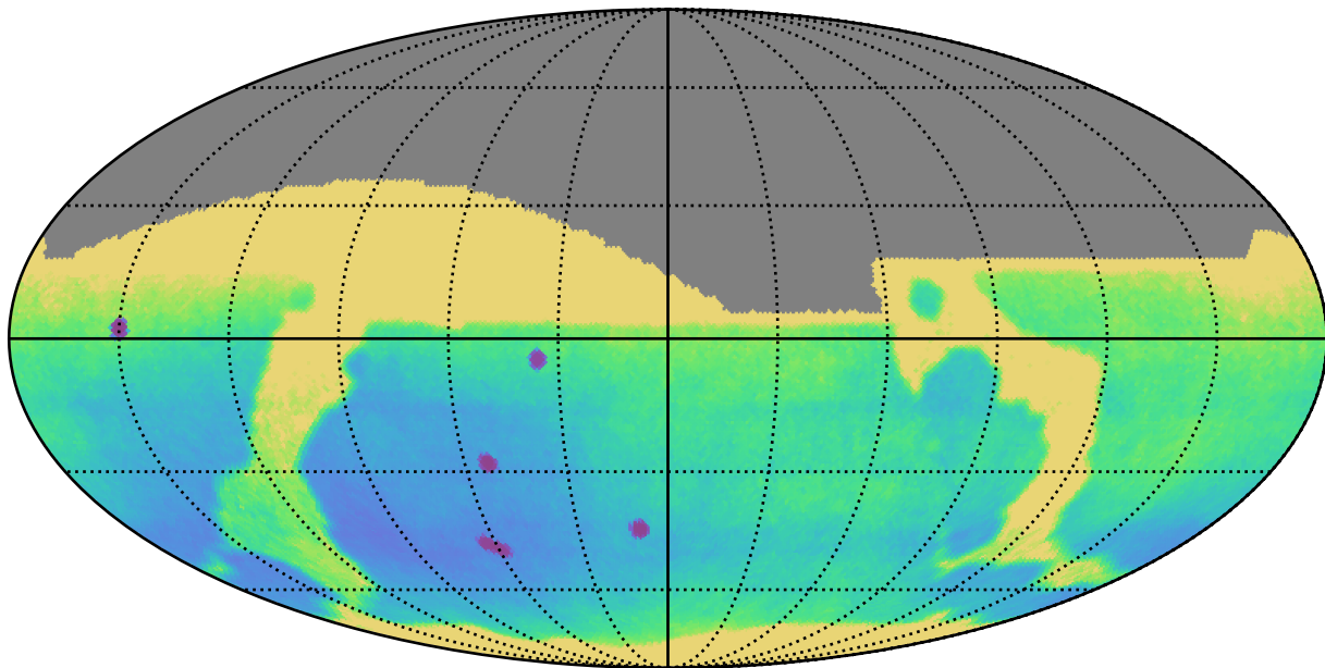
weather_cloudso36v3.4_10yrs : Parallax Uncert @ 24.0
