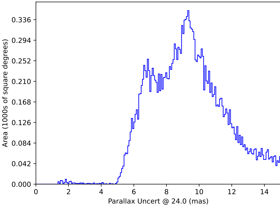
weather_cloudso36v3.4_10yrs : Parallax Uncert @ 24.0
