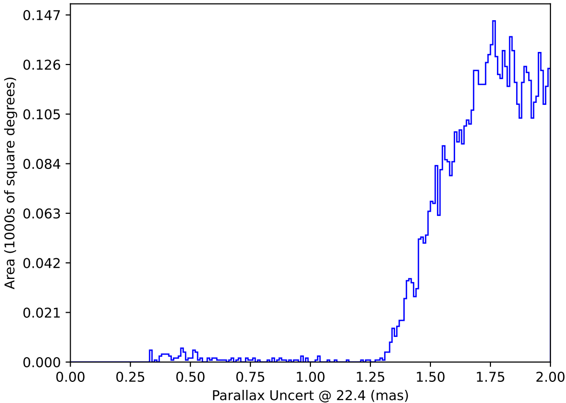
weather_cloudso36v3.4_10yrs : Parallax Uncert @ 22.4
