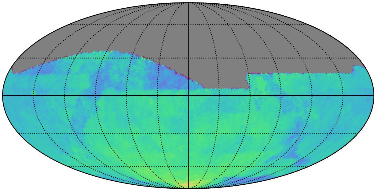
weather_cloudso36v3.4_10yrs : Parallax Coverage @ 24.0
