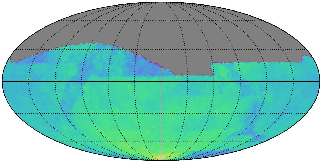
weather_cloudso36v3.4_10yrs : Parallax Coverage @ 22.4
