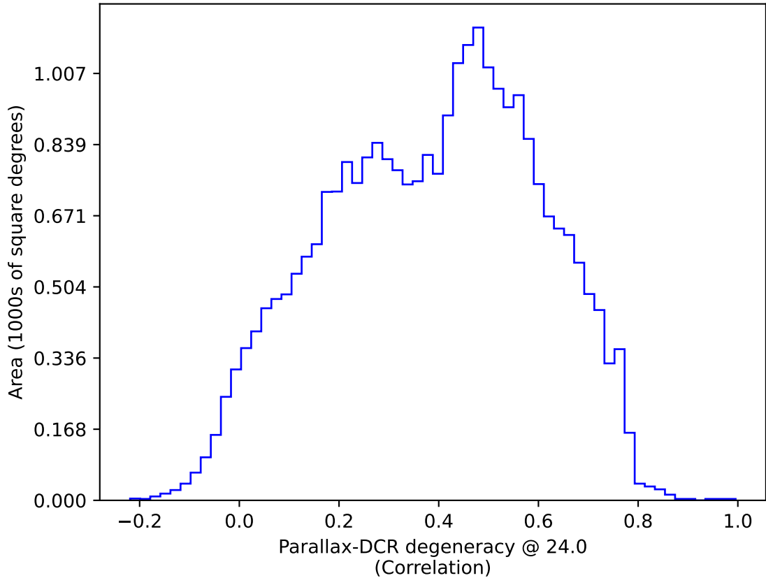
weather_cloudso36v3.4_10yrs : Parallax-DCR degeneracy @ 24.0
