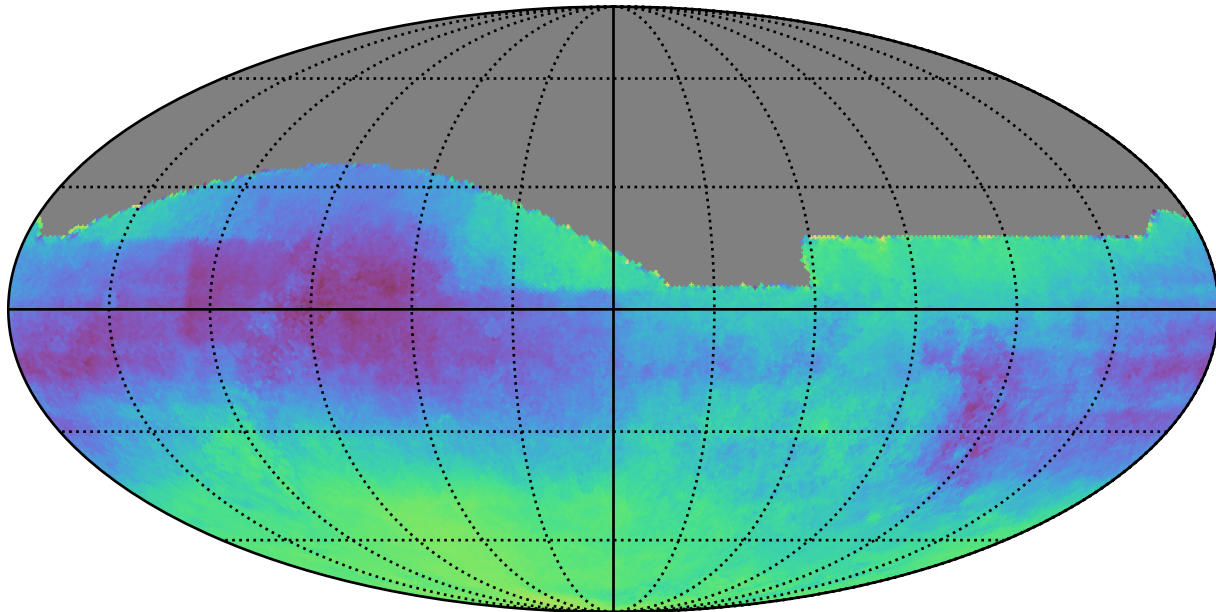
weather_cloudso36v3.4_10yrs : Parallax-DCR degeneracy @ 22.4
