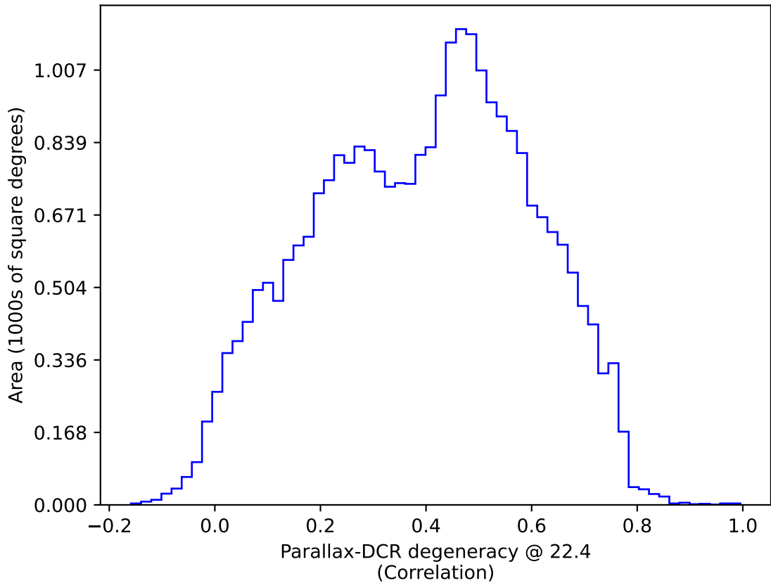
weather_cloudso36v3.4_10yrs : Parallax-DCR degeneracy @ 22.4
