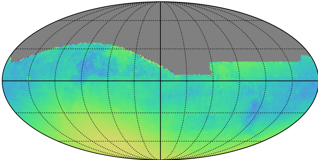
weather_cloudso36v3.4_10yrs : Normalized Parallax Uncert @ 24.0
