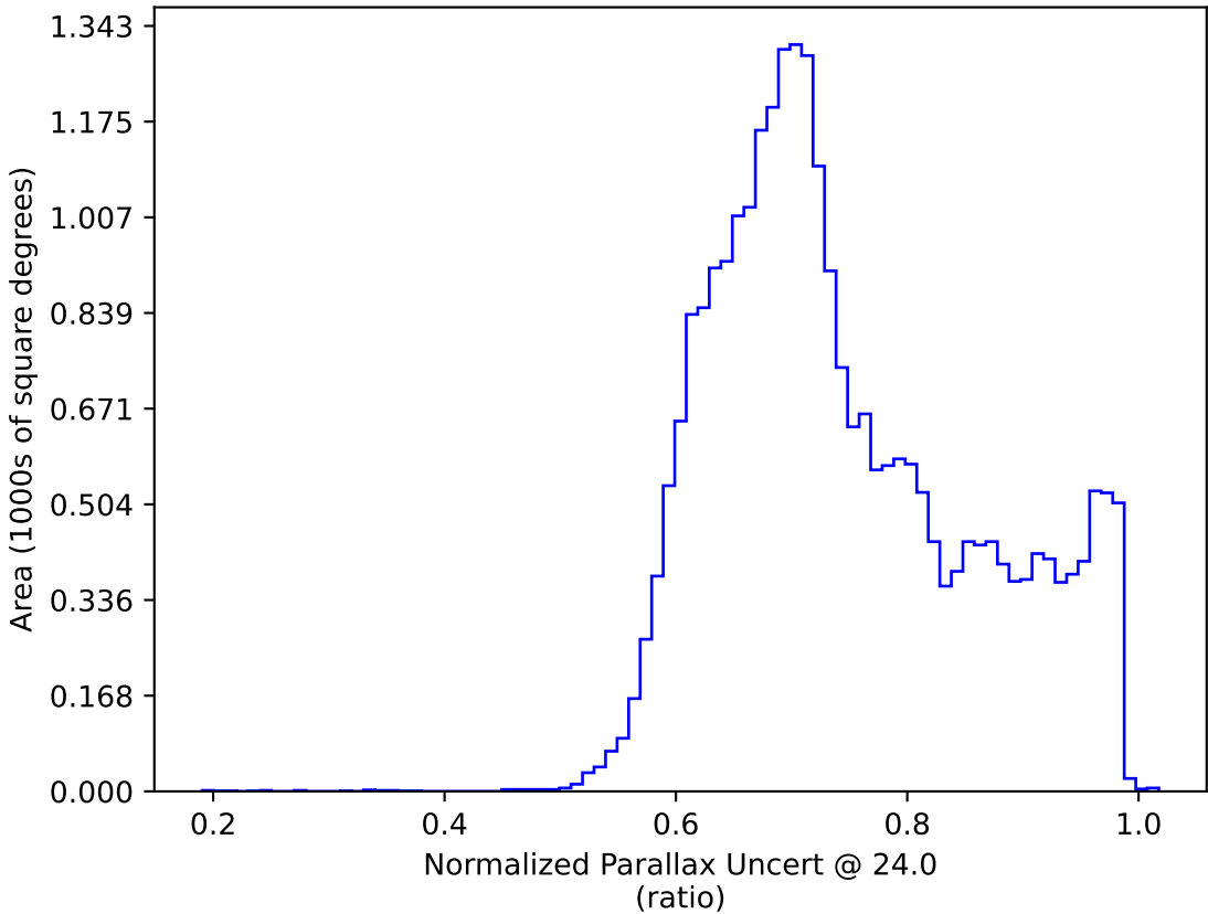
weather_cloudso36v3.4_10yrs : Normalized Parallax Uncert @ 24.0
