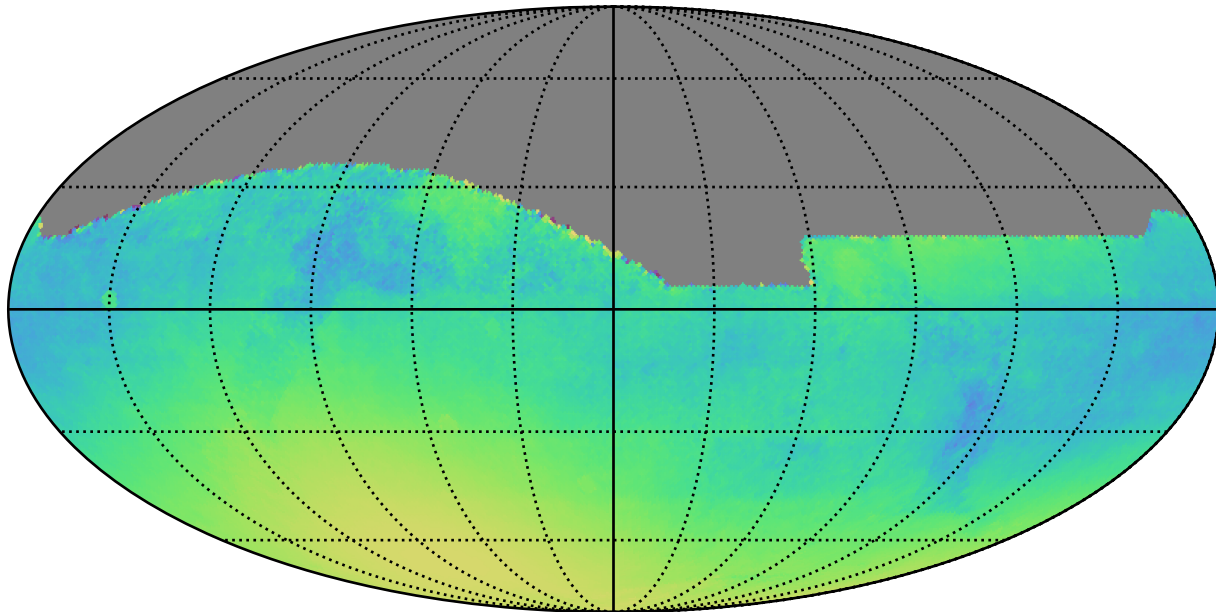
weather_cloudso36v3.4_10yrs : Normalized Parallax Uncert @ 22.4
