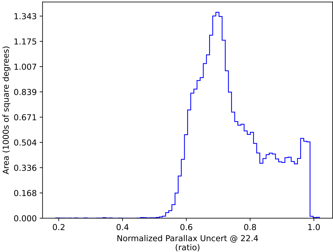
weather_cloudso36v3.4_10yrs : Normalized Parallax Uncert @ 22.4
