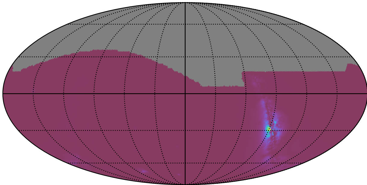
weather_cloudso36v3.4_10yrs : NlcPoints
