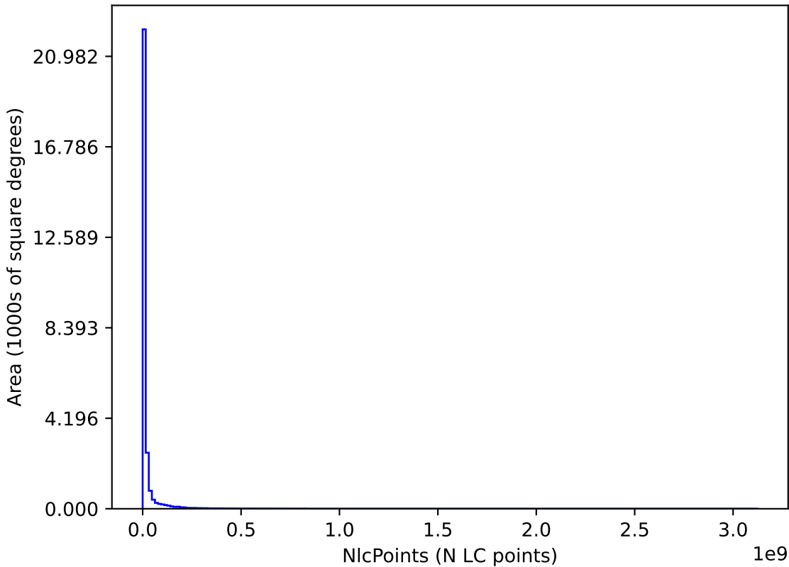
weather_cloudso36v3.4_10yrs : NlcPoints
