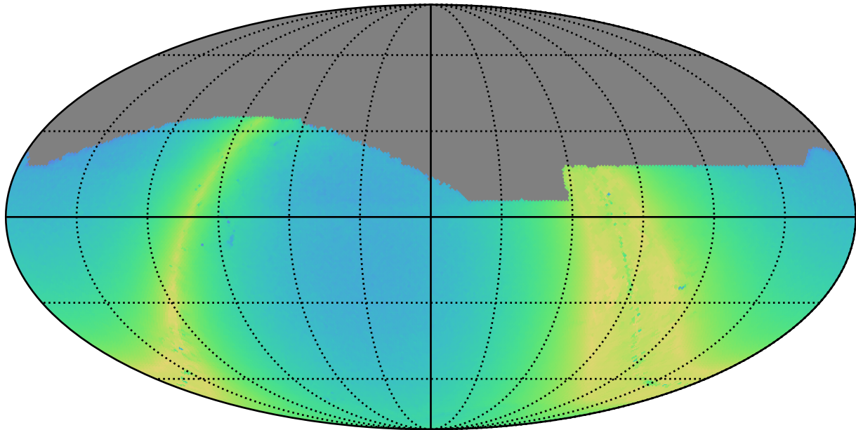
weather_cloudso36v3.4_10yrs z: N stars to Precision 0.20
