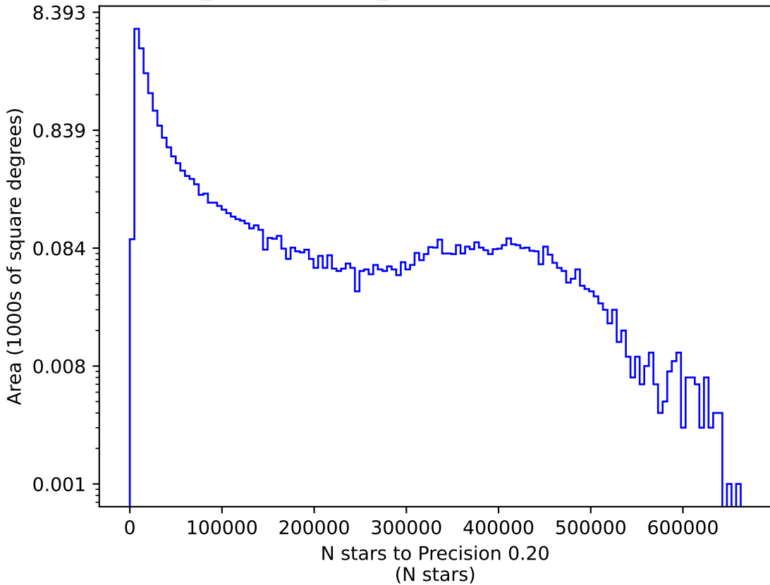
weather_cloudso36v3.4_10yrs z: N stars to Precision 0.20
