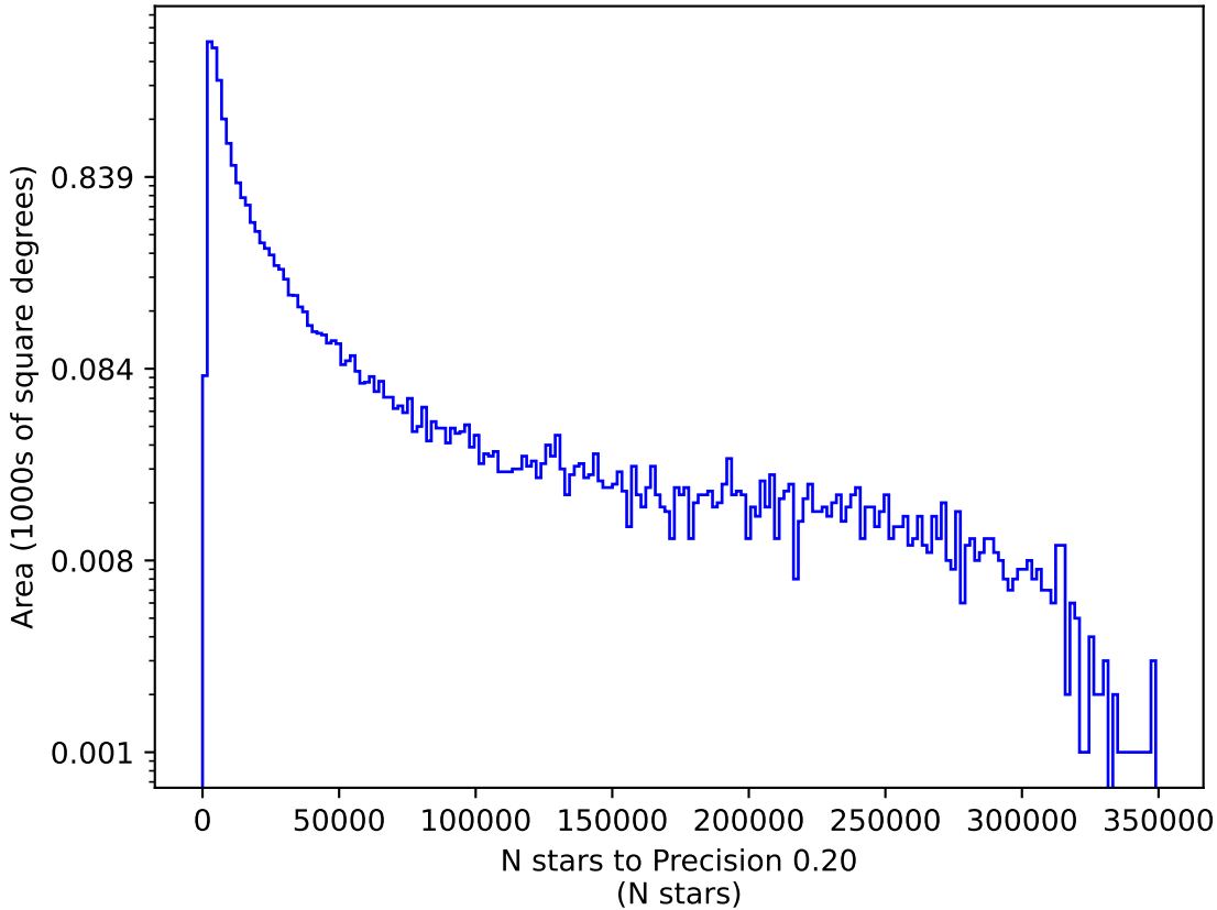
weather_cloudso36v3.4_10yrs u: N stars to Precision 0.20
