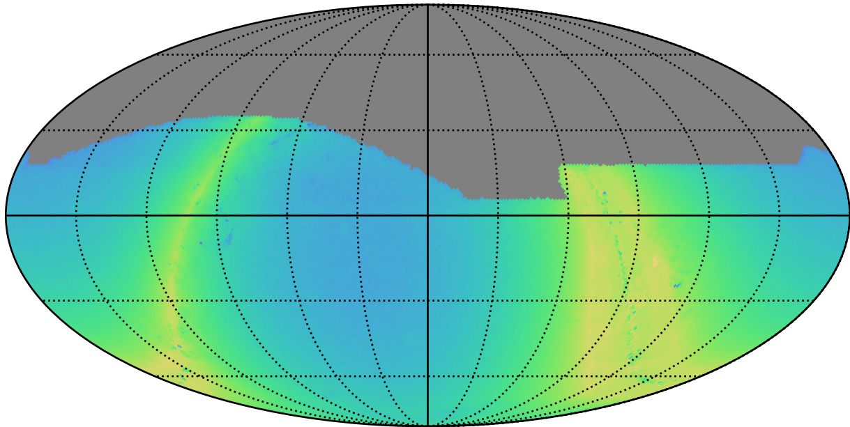
weather_cloudso36v3.4_10yrs r: N stars to Precision 0.20
