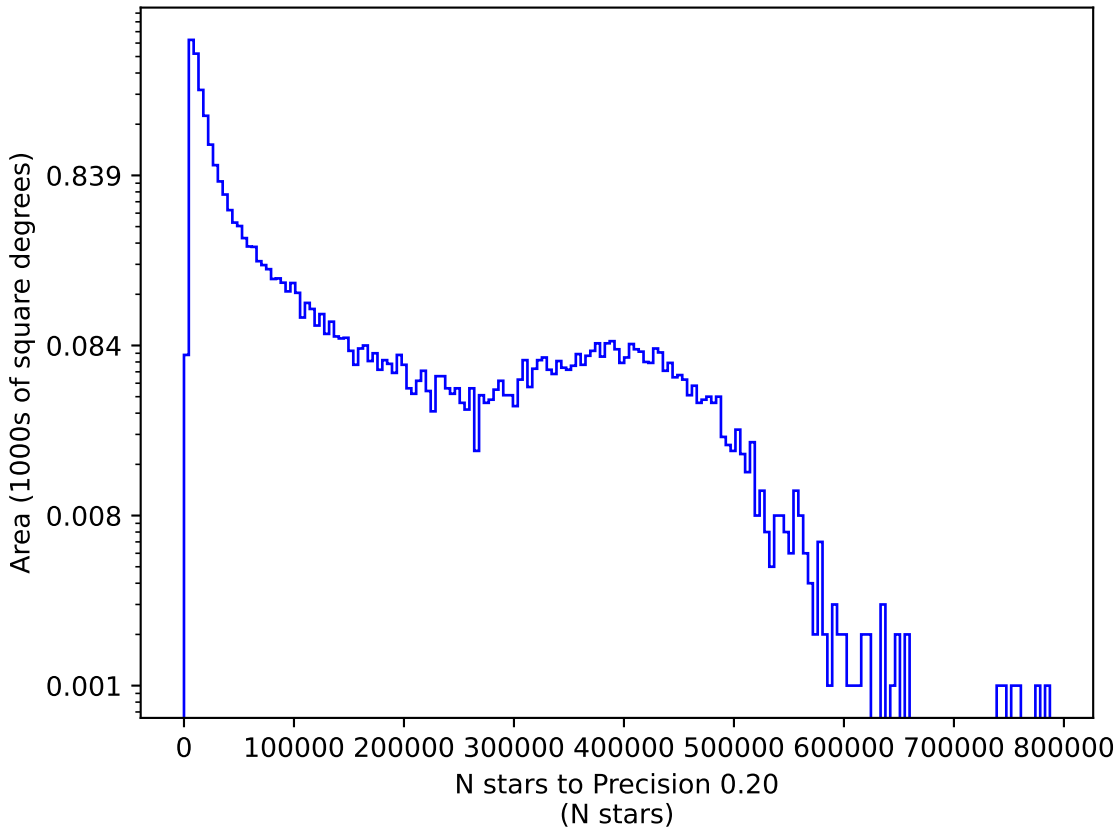
weather_cloudso36v3.4_10yrs r: N stars to Precision 0.20
