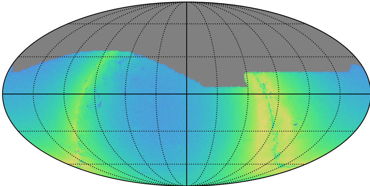
weather_cloudso36v3.4_10yrs g: N stars to Precision 0.20
