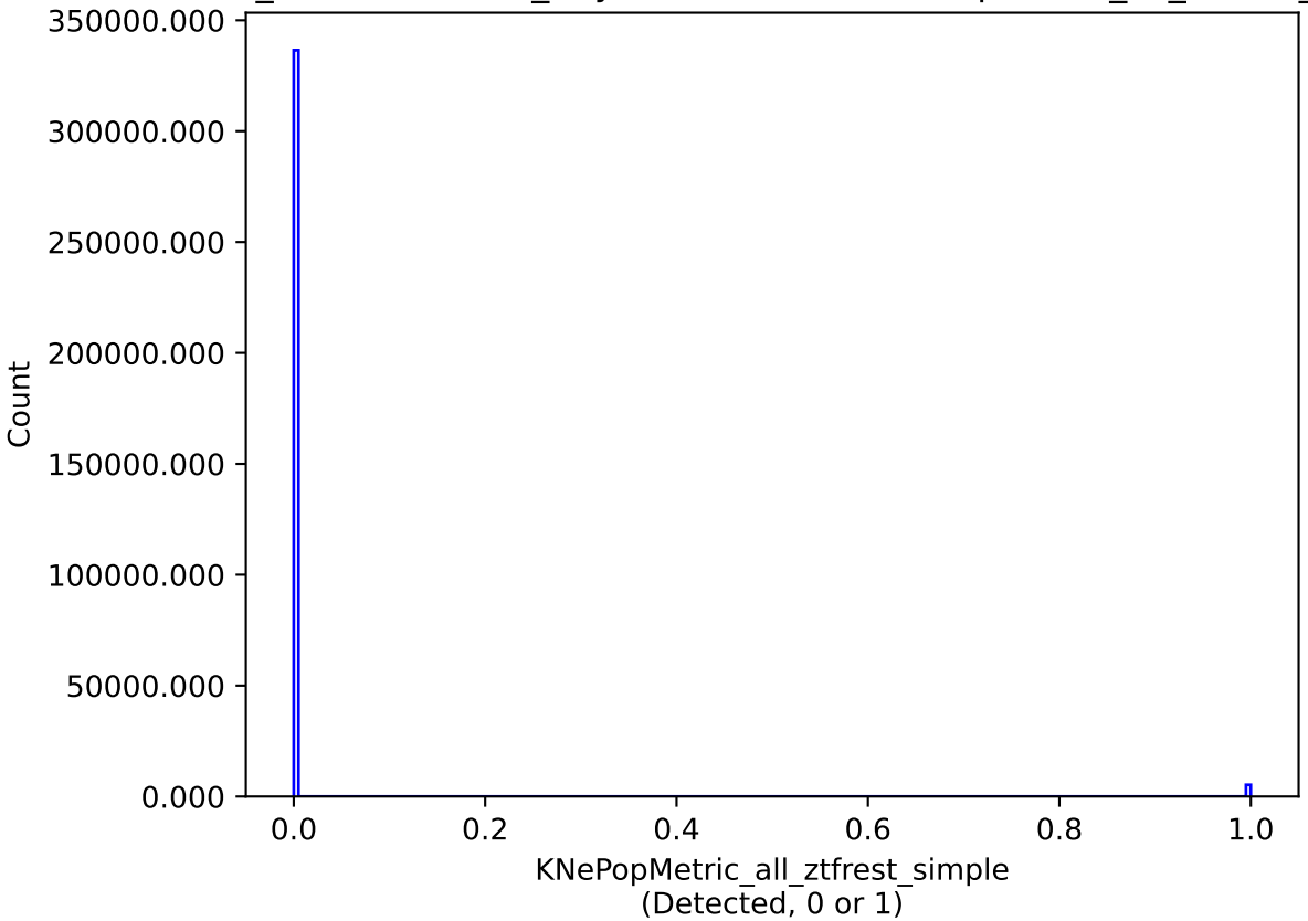
weather_cloudso36v3.4_10yrs all models: KNePopMetric_all_ztfrest_simple
