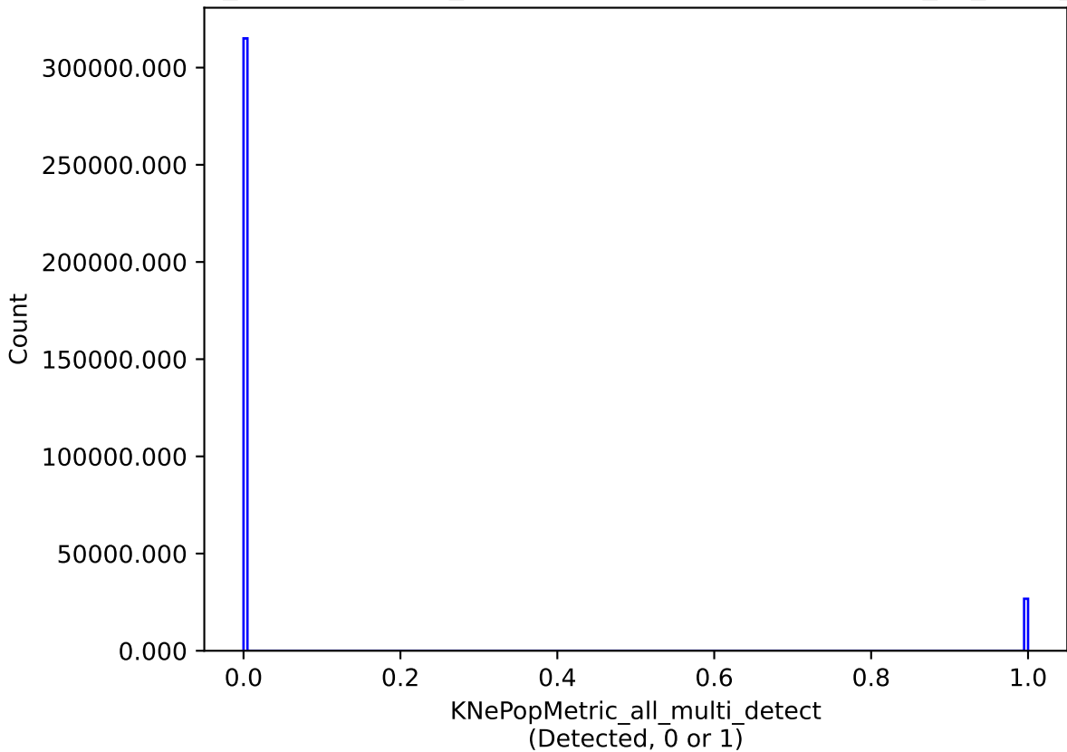
weather_cloudso36v3.4_10yrs all models: KNePopMetric_all_multi_detect
