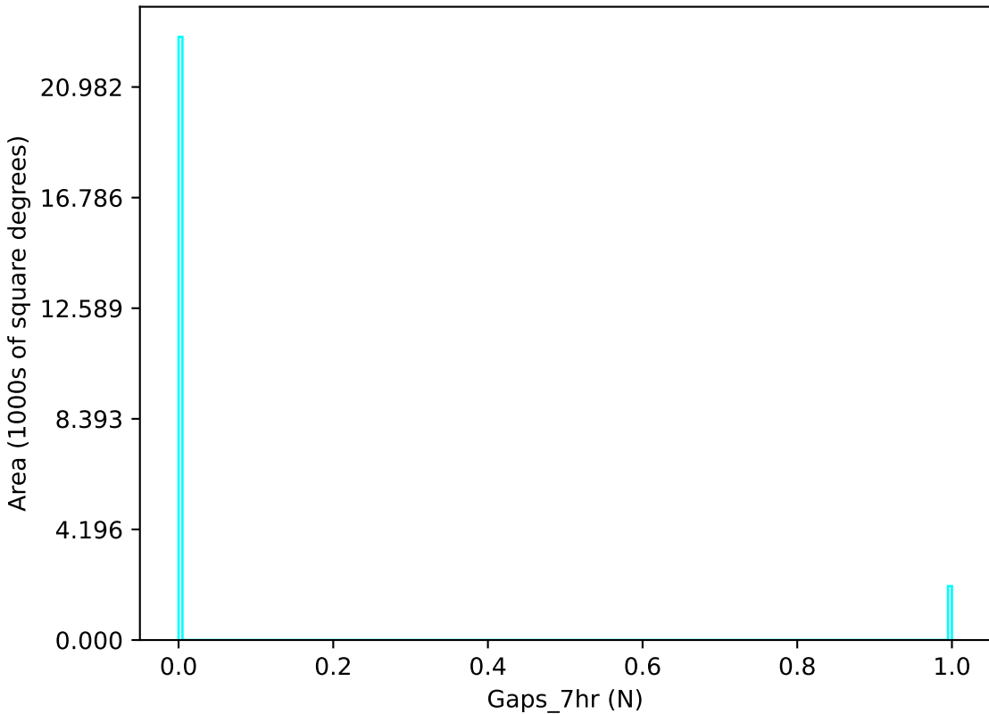
weather_cloudso36v3.4_10yrs u band: Gaps_7hr
