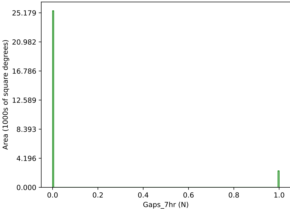
weather_cloudso36v3.4_10yrs g band: Gaps_7hr
