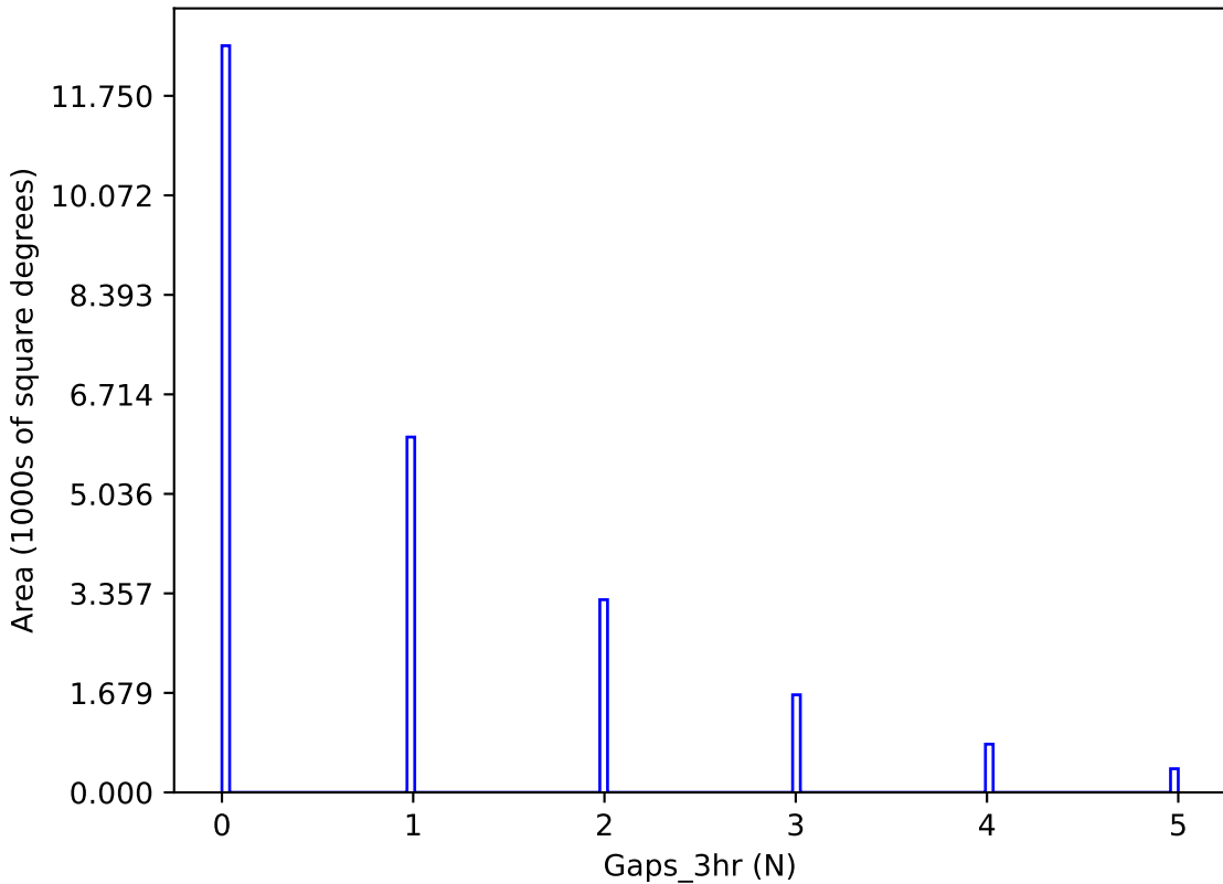
weather_cloudso36v3.4_10yrs y band: Gaps_3hr
