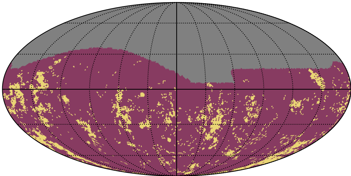
weather_cloudso36v3.4_10yrs g band: Gaps_3hr
