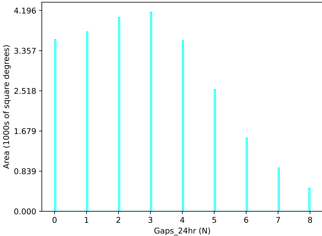
weather_cloudso36v3.4_10yrs u band: Gaps_24hr
