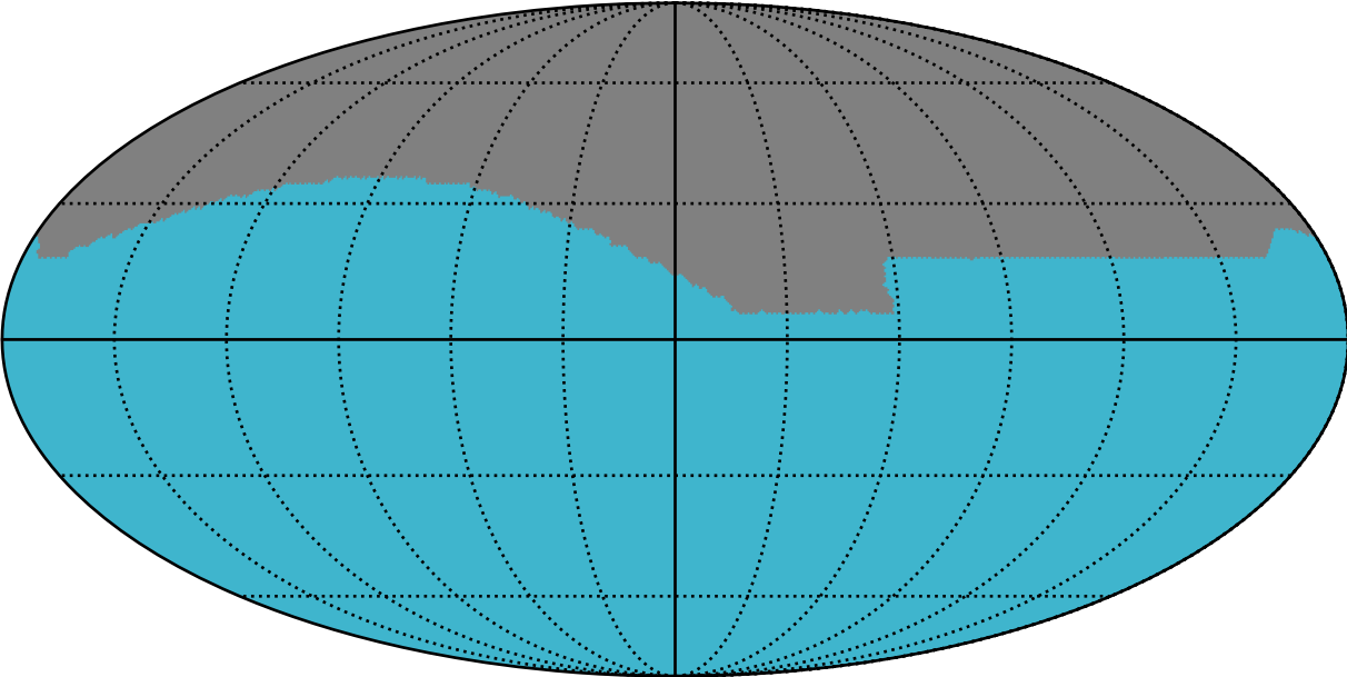
weather_cloudso36v3.4_10yrs : GalplaneFootprintMetric_xray_binaries_map_Tau_2_0
