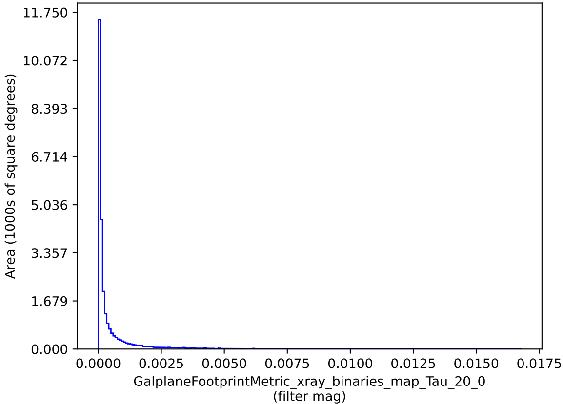
weather_cloudso36v3.4_10yrs : GalplaneFootprintMetric_xray_binaries_map_Tau_20_0
