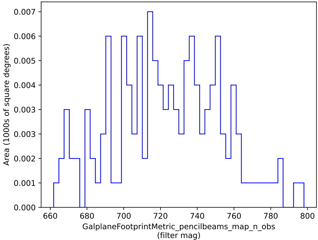
weather_cloudso36v3.4_10yrs : GalplaneFootprintMetric_pencilbeams_map_n_obs
