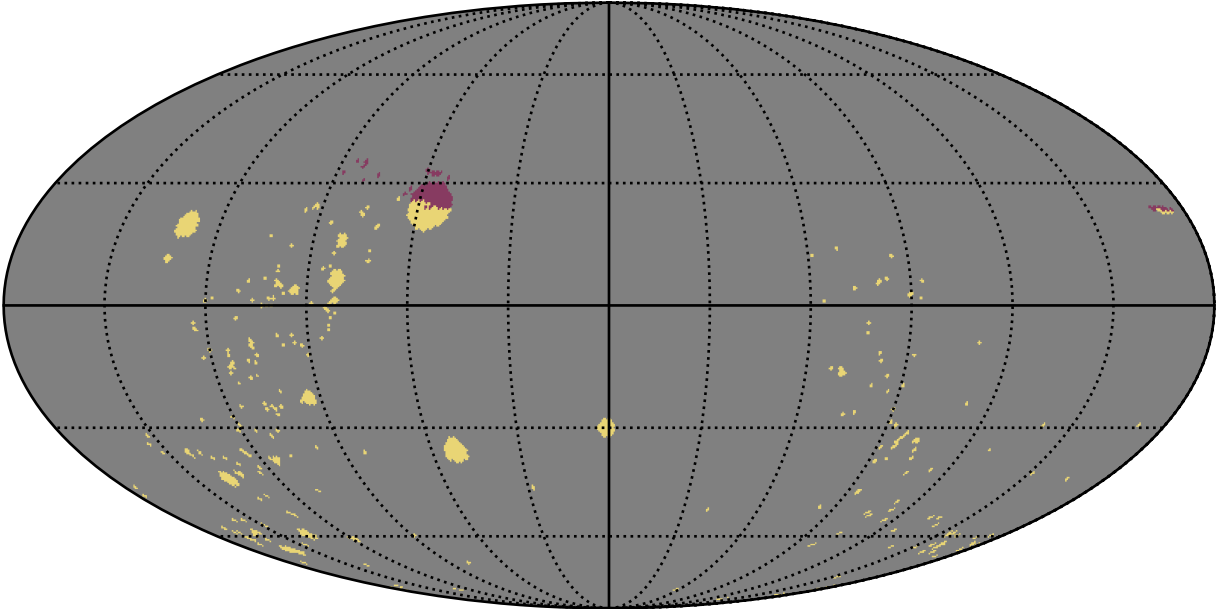
weather_cloudso36v3.4_10yrs : GalplaneFootprintMetric_open_clusters_map_Tau_73_0
