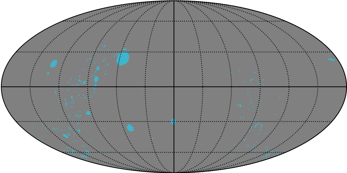
weather_cloudso36v3.4_10yrs : GalplaneFootprintMetric_open_clusters_map_Tau_2_0
