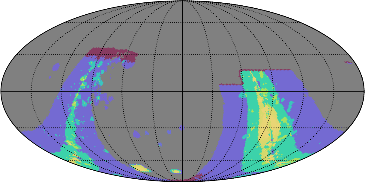
weather_cloudso36v3.4_10yrs : GalplaneFootprintMetric_combined_map_Tau_73_0
