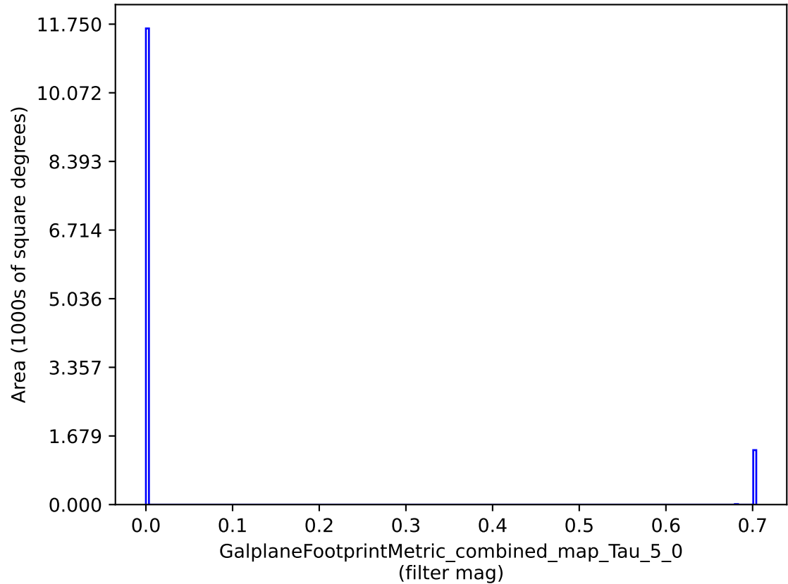
weather_cloudso36v3.4_10yrs : GalplaneFootprintMetric_combined_map_Tau_5_0
