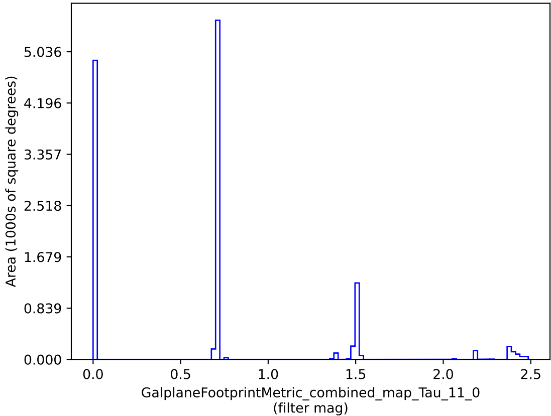
weather_cloudso36v3.4_10yrs : GalplaneFootprintMetric_combined_map_Tau_11_0
