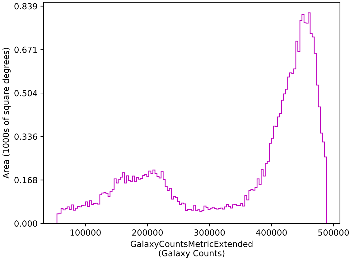
weather_cloudso36v3.4_10yrs z: GalaxyCountsMetricExtended
