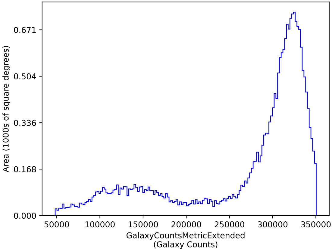
weather_cloudso36v3.4_10yrs y: GalaxyCountsMetricExtended
