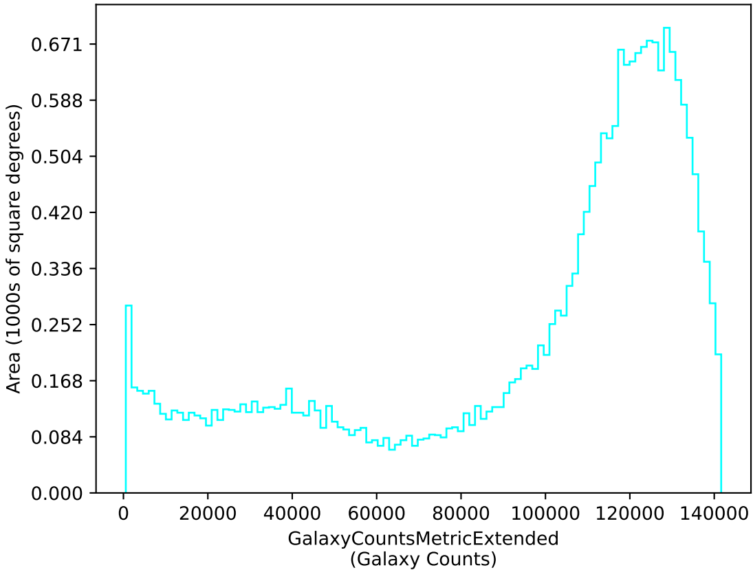
weather_cloudso36v3.4_10yrs u: GalaxyCountsMetricExtended
