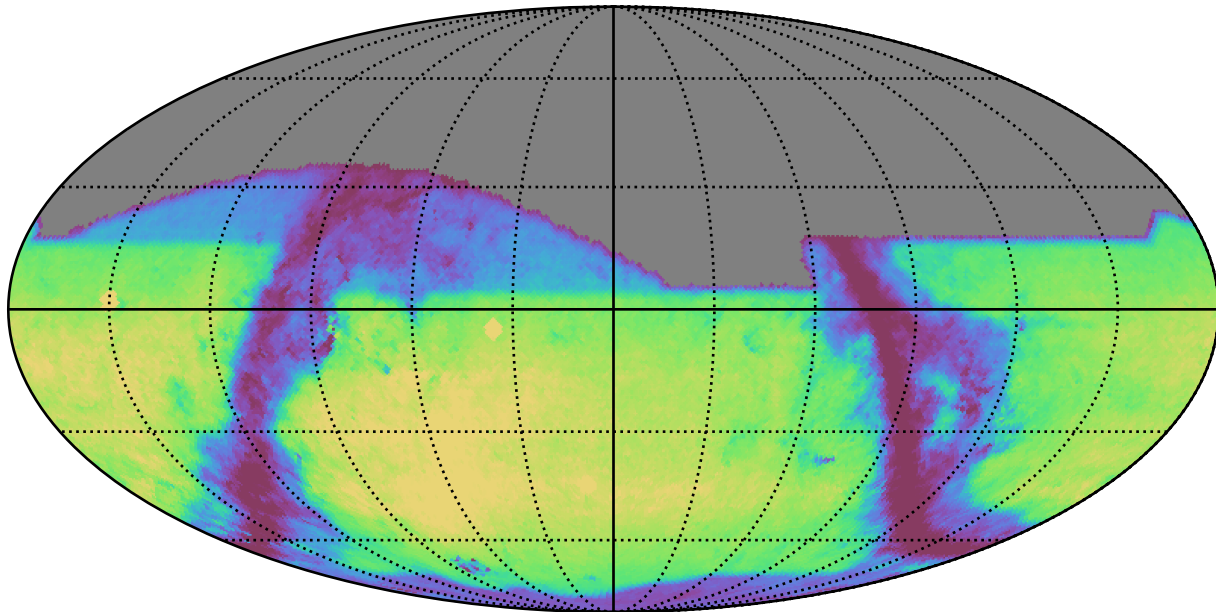
weather_cloudso36v3.4_10yrs r: GalaxyCountsMetricExtended
