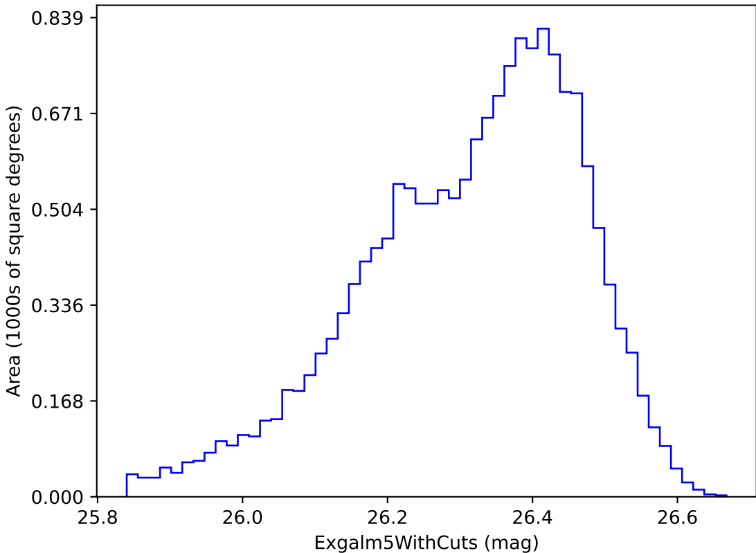
weather_cloudso36v3.4_10yrs i band non-DD year 9: ExgalM5WithCuts
