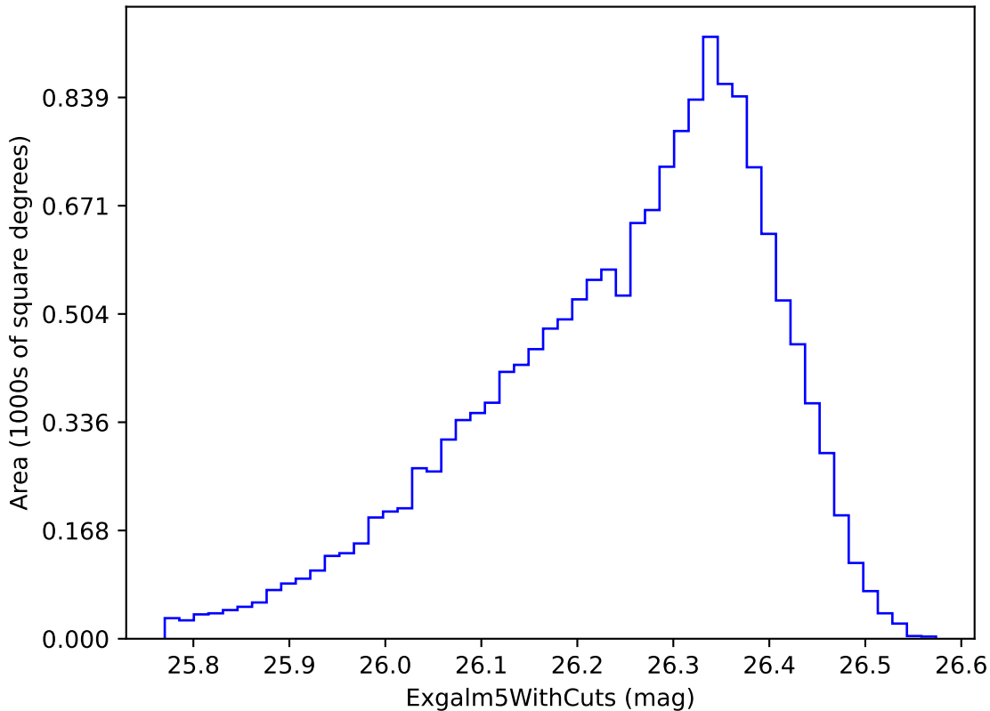
weather_cloudso36v3.4_10yrs i band non-DD year 8: ExgalM5WithCuts
