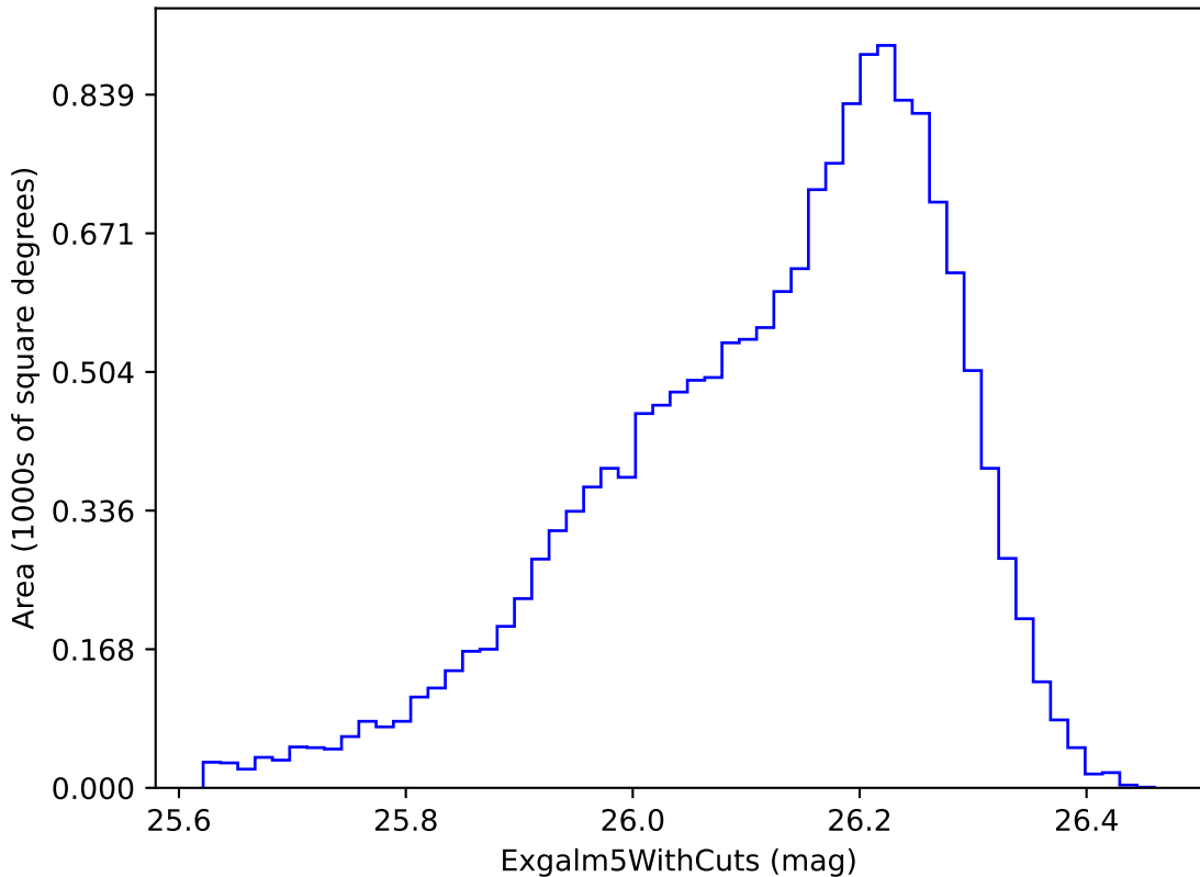
weather_cloudso36v3.4_10yrs i band non-DD year 6: ExgalM5WithCuts
