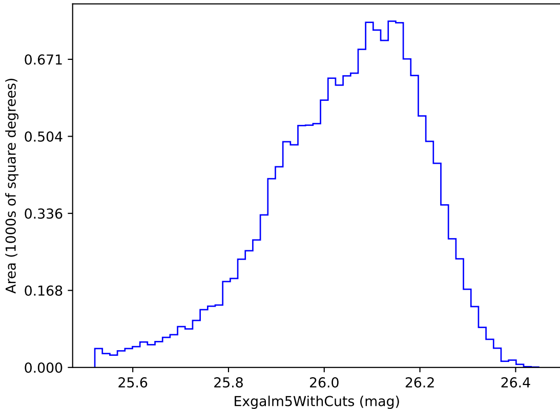
weather_cloudso36v3.4_10yrs i band non-DD year 5: ExgalM5WithCuts
