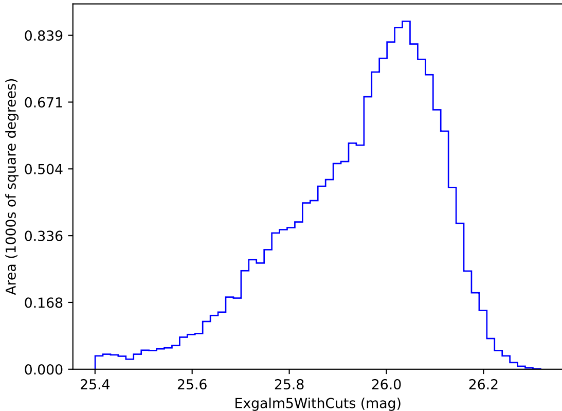
weather_cloudso36v3.4_10yrs i band non-DD year 4: Exgalml5WithCuts
