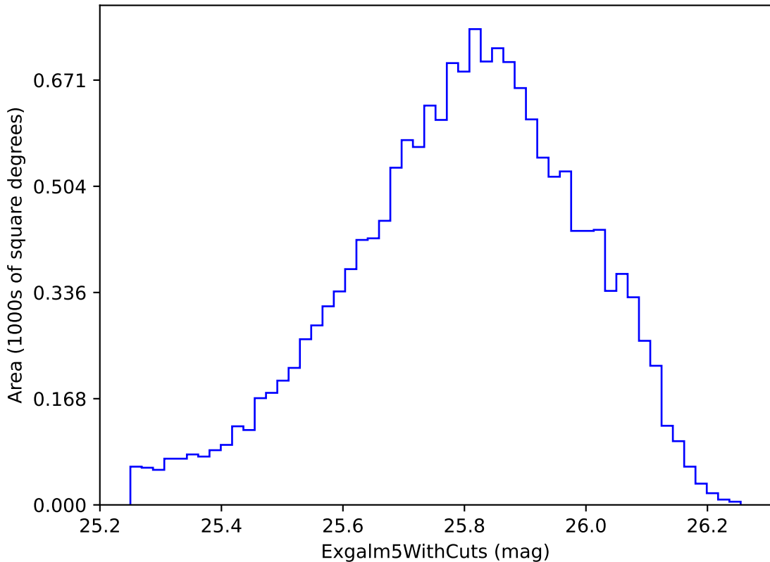
weather_cloudso36v3.4_10yrs i band non-DD year 3: ExgalM5WithCuts
